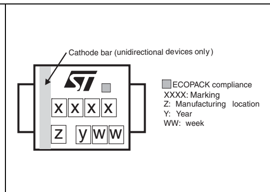
Figure 18. Marking layout (1)
