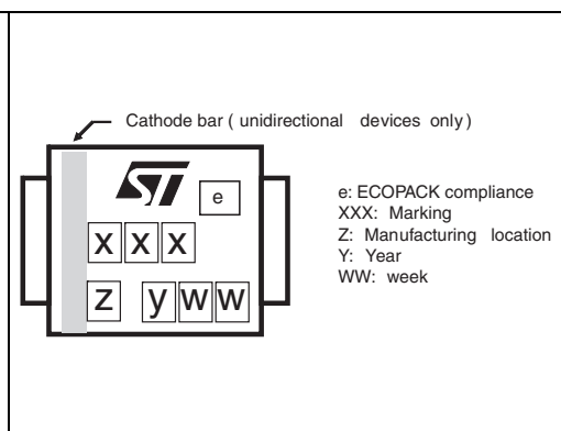
Figure 14. Marking layout (1)
