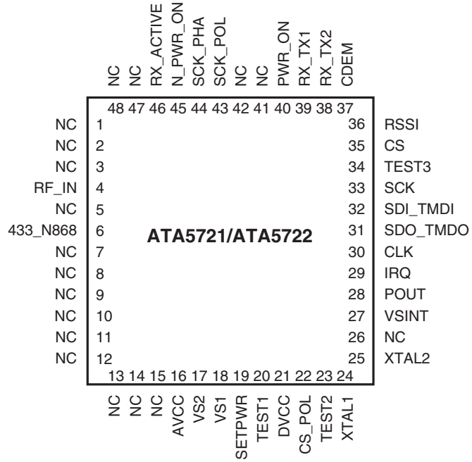
Figure 1-1. Pinning QFN48
