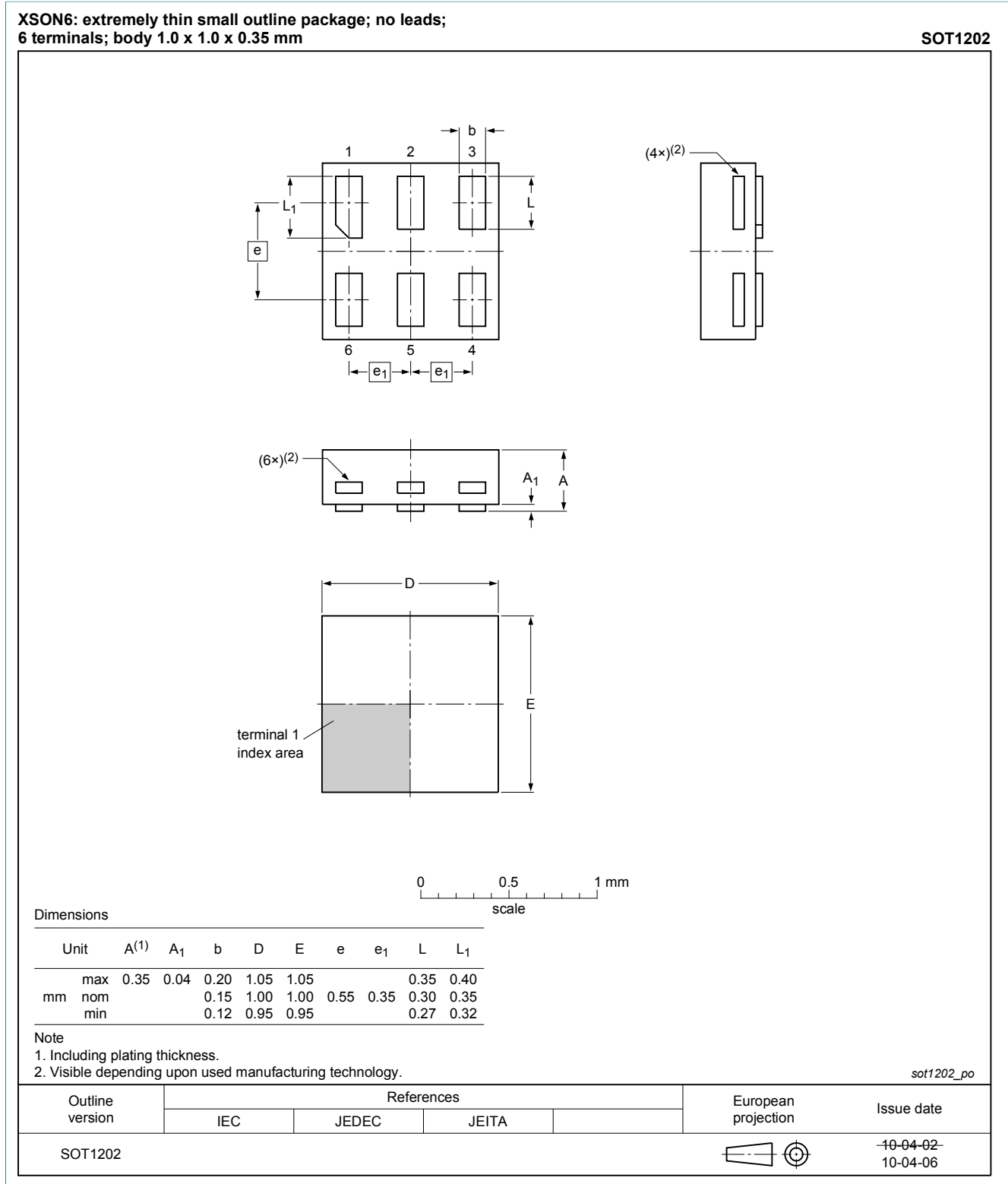
Figure 21. Package outline SOT1202 (XSON6)
