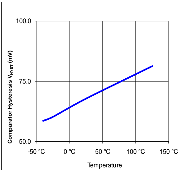
Figure 19: Comparator Hysteresis vs. Temperature
