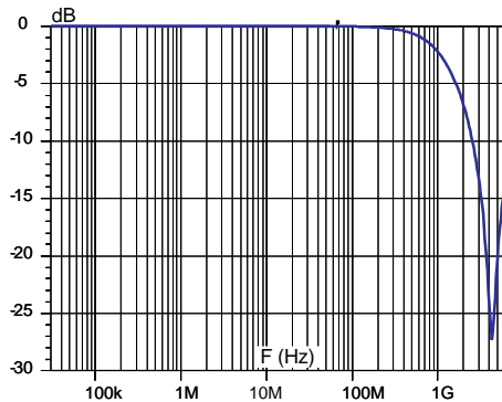
Figure 13: S21 attenuation measurement result
