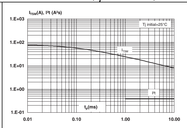
Figure 6. Non repetitive surge peak on-state current for a sinusoidal pulse with width t_p < 10 ms, and corresponding value of I^2t ( T_j \text{ initial} = 25^\circ\text{C} ).
