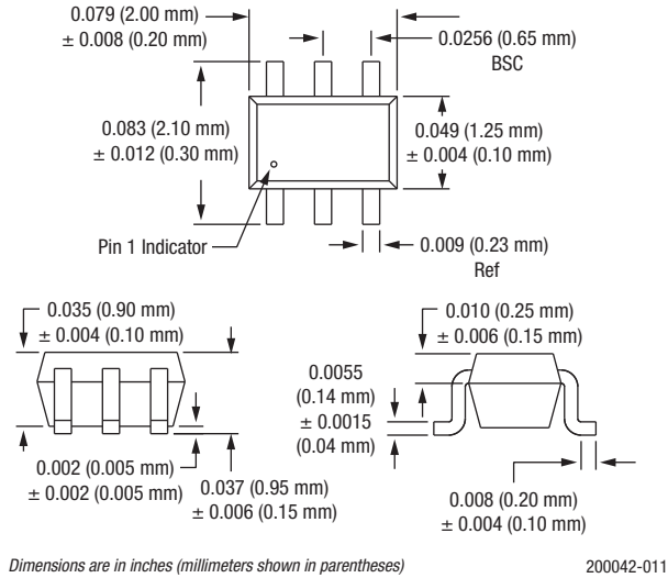
Figure 9. SC-88 Package Dimension Drawing
