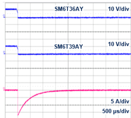
Figure 13. ISO7637-2 pulse 1: V_s = -150 V with 12 V battery
