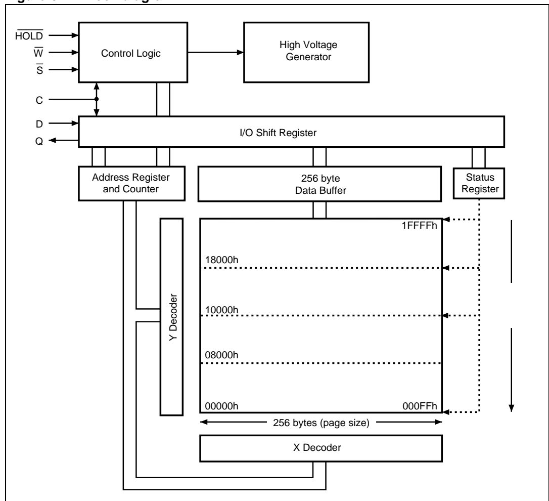
Figure 6. Block diagram
