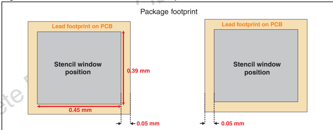
Figure 16. Recommended stencil windows position
