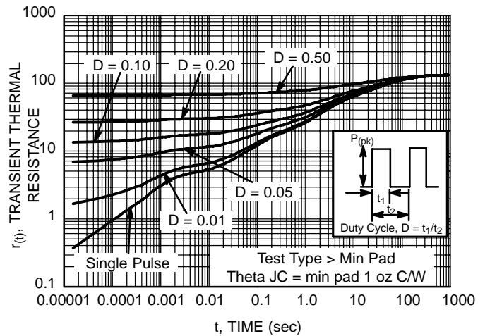
Figure 8. Thermal Response
