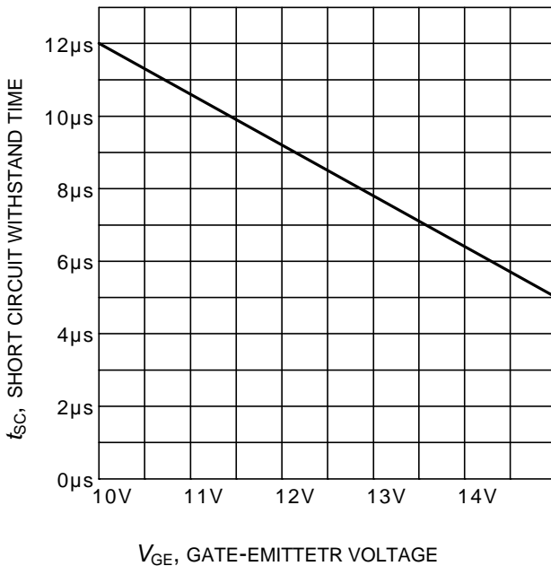
Figure 19. Short circuit withstand time as a function of gate-emittetr voltage ( V_{CE}=400\text{V} , start at T_J=25^\circ\text{C} , T_{Jmax}<150^\circ\text{C} )
