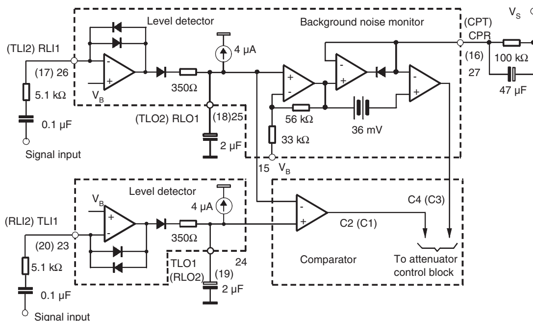
Figure 3-2. Level Detectors
