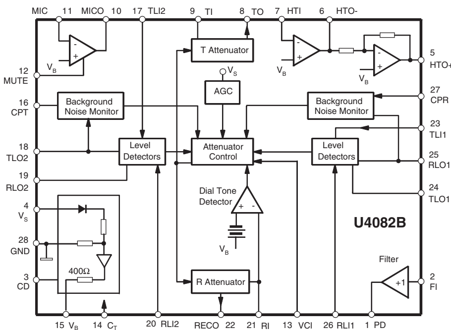
Figure 1-1. Block Diagram
