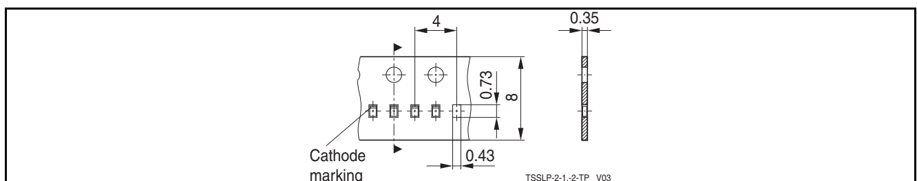
Figure 13 PG-TSSLP-2-1: Packing
