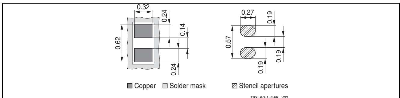
Figure 12 PG-TSSLP-2-1: Footprint
