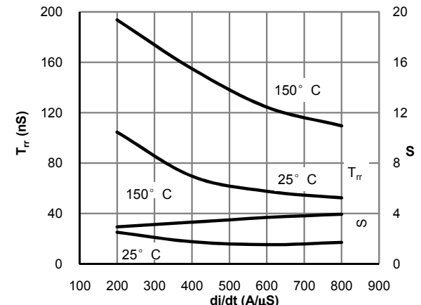
Fig 25: Diode Reverse Recovery Time and Softness Factor vs. di/dt ( V_{GE}=15V, V_{CE}=400V, I_F=10A )
