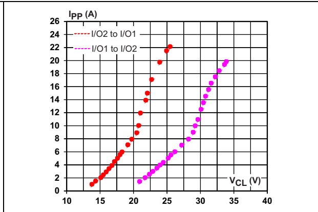
Figure 12. TLP measurements
