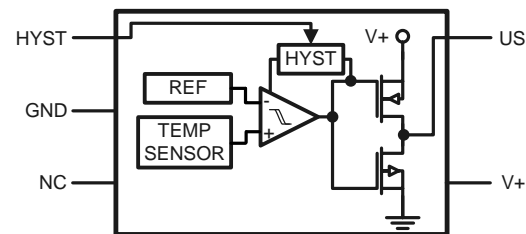
Figure 4. LM26CIM5 - __ F
