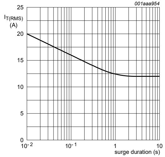
f = 50 Hz; T_{mb} = 103\text{ }^{\circ}\text{C} Fig. 3. RMS on-state current as a function of surge duration; maximum values
