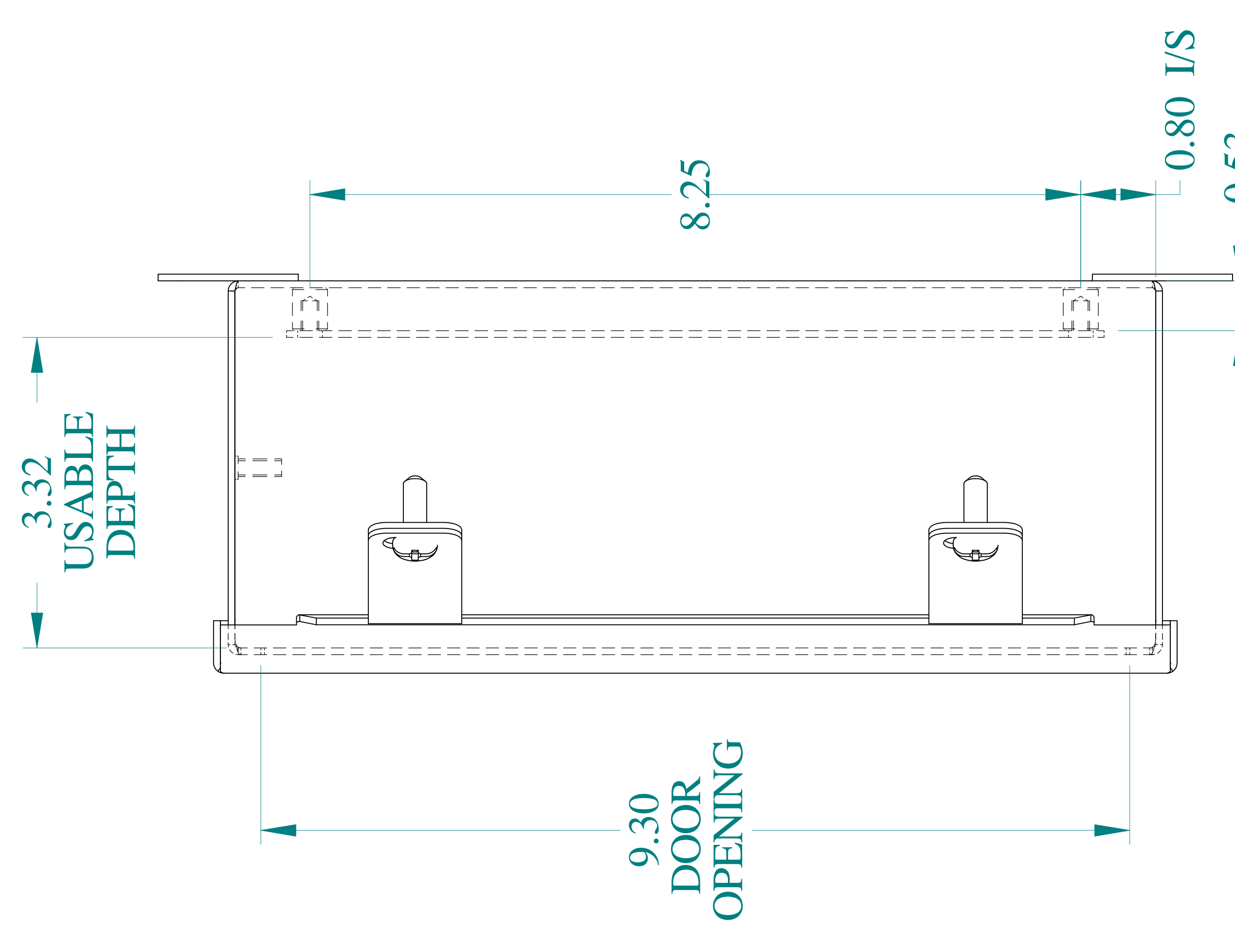
SIDE VIEW
