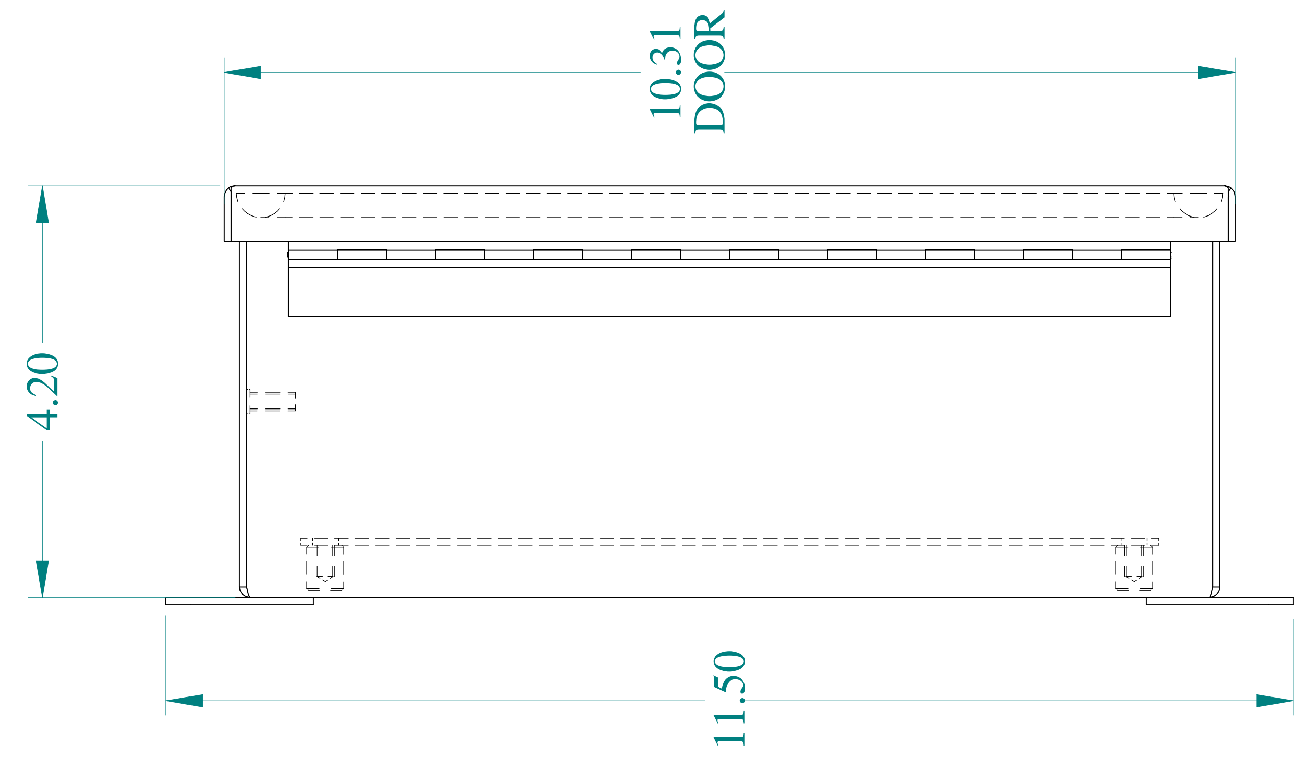
SIDE VIEW
