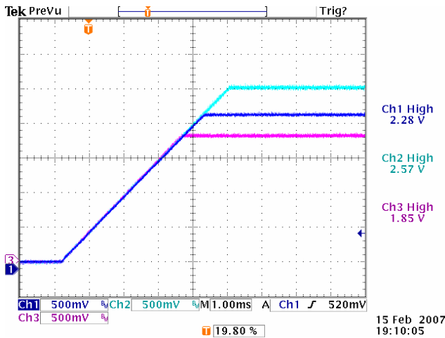
Figure 7. Tracking Turn-On. Rising Slew Rate is Programmed at 0.5V/ms. Vin=12V, Ch1 – V1, Ch2 – V2, Ch3 – V3
