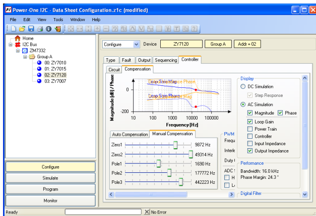
Figure 47. POL Configure Controller Compensation Window
