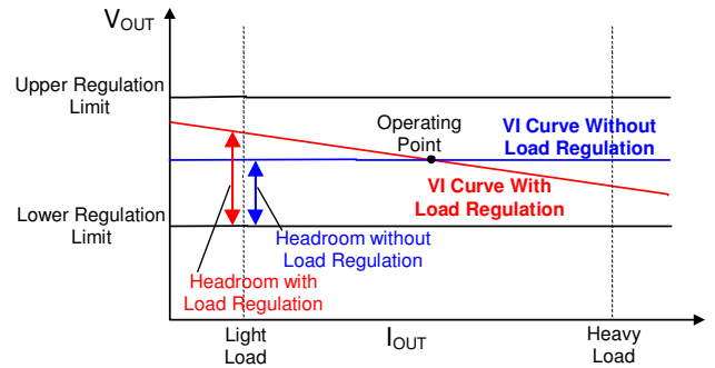
Figure 9. Optimal Voltage Positioning Concept
