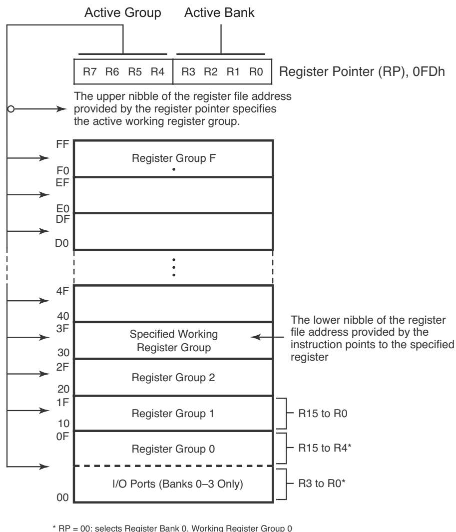
Figure 10. Register Pointer—Detail
