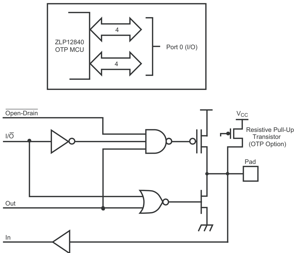
Figure 4. Port 0 Configuration
