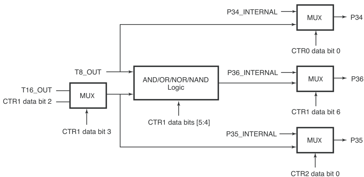
Figure 30. Output Circuit
