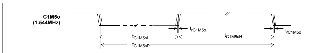
Figure 29 - C1M5o Output Clock Timing Diagram
