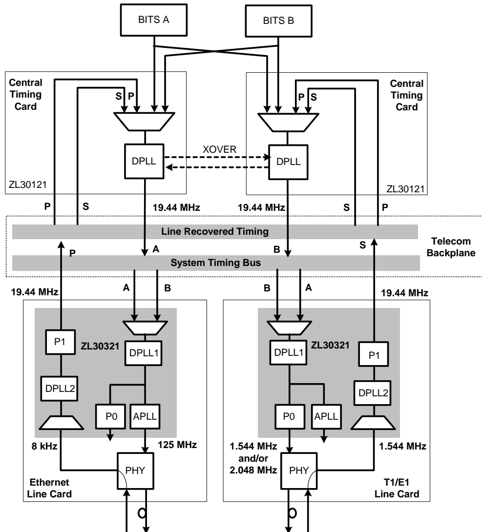
Figure 2 - Typical Application of the ZL30321
