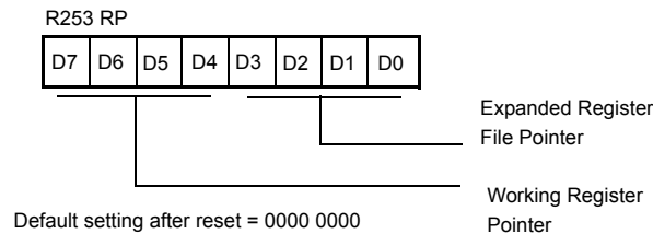
Figure 23. Register Pointer
