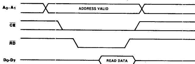
Figure 8-3. Z8536 (CIO) Read Cycle Timing
