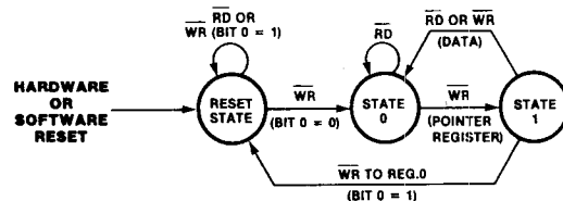
Figure 2-1. Z8536 State Machine Operation
