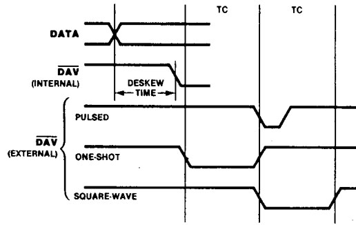
Figure 3-12. Pulsed Output Handshake Counter/Timer Duty Cycles
