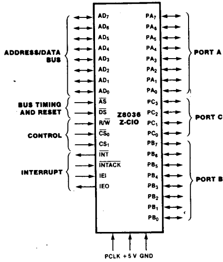
Figure 1. Pin Functions
