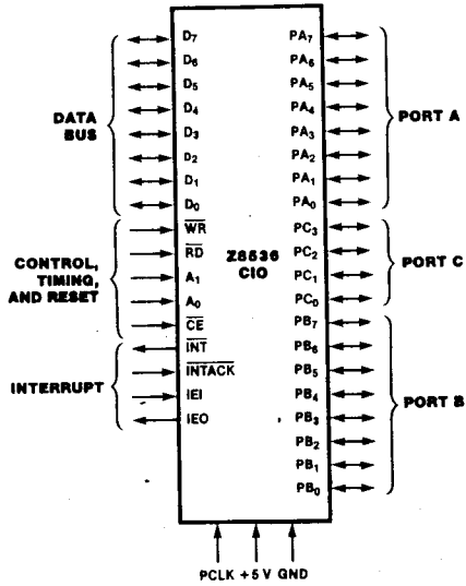
Figure 1. Pin Functions
