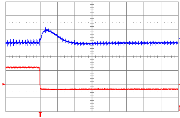
Fig. 1.8V.7: Output voltage response for V_{out} = 1.8V to negative load current step change from 16A to 8A with slew rate of -5A/ \mu s at V_{in} = 12V . Top trace: output voltage (200mV/div.); Bottom trace: load current (5A/div.). C_o = 100\mu F ceramic. Time scale: 20 \mu s/div.
