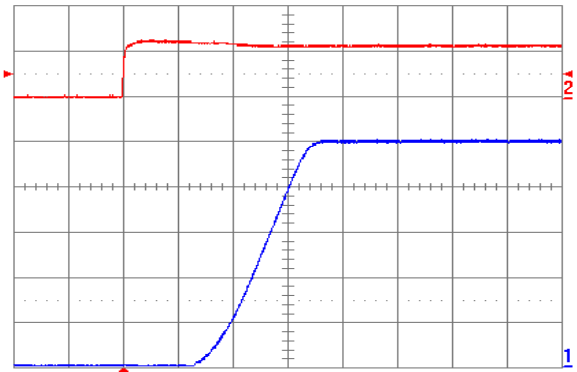
Fig. 5.0V.4: Turn-on transient for V_{out} = 5.0V with application of V_{in} at full rated load current (resistive) and 100\mu F external capacitance at V_{in} = 12V . Top trace: V_{in} (10V/div.); Bottom trace: output voltage (1V/div.); Time scale: 2ms/div.
