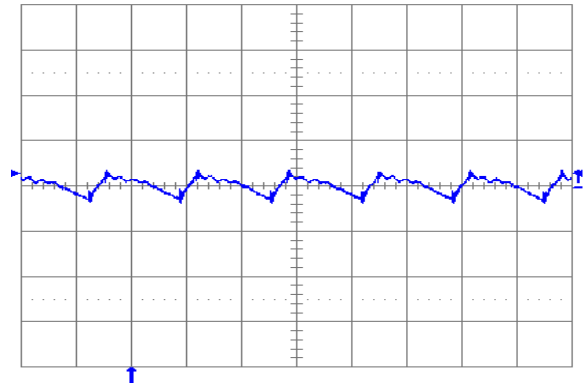
Fig. 2.0V.6: Output voltage ripple (20 mV/div.) at full rated load current into a resistive load with external capacitance 100 \mu F ceramic + 1 \mu F ceramic, and V_{in} = 12 V for V_{out} = 2.0 V. Time scale: 2 \mu s/div.
