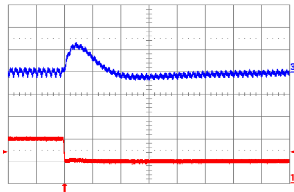
Fig. 2.5V.8: Output voltage response for V_{out} = 2.5 V to negative load current step change from 10 A to 5 A with slew rate of -5 A/ \mu s at V_{in} = 12 V. Top trace: output voltage (100 mV/div.); Bottom trace: load current (5 A/div.). C_o = 100 \mu F ceramic. Time scale: 20 \mu s/div.
