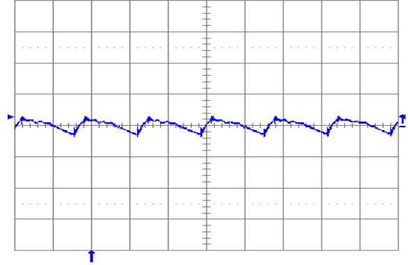
Fig. 1.8V.6: Output voltage ripple (20 mV/div.) at full rated load current into a resistive load with external capacitance 100\ \mu\text{F} ceramic + 1\ \mu\text{F} ceramic, and V_{in} = 12\text{ V} for V_{out} = 1.8\text{ V} . Time scale: 2\ \mu\text{s}/\text{div} .
