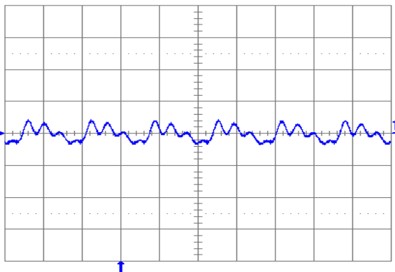
Fig. 1.8V.5: Output voltage ripple (20 mV/div.) at full rated load current into a resistive load with external capacitance 100\text{ }\mu\text{F} ceramic + 1\text{ }\mu\text{F} ceramic and V_{in} = 12\text{ V} for V_{out} = 1.8\text{ V} . Time scale: 2\text{ }\mu\text{s}/\text{div} .
