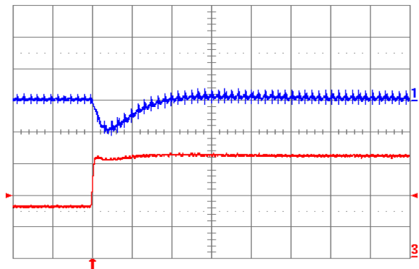
Fig. 1.8V.6: Output voltage response for V_{out} = 1.8\text{ V} to positive load current step change from 8 A to 16 A with slew rate of 5\text{ A}/\mu\text{s} at V_{in} = 12\text{ V} . Top trace: output voltage (200 mV/div.); Bottom trace: load current (5 A/div.). C_o = 100\text{ }\mu\text{F} ceramic. Time scale: 20\text{ }\mu\text{s}/\text{div} .
