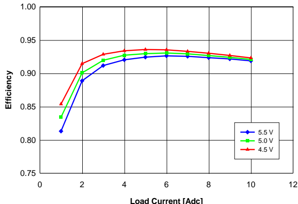
Fig. 2.0V.3: Efficiency vs. load current and input voltage for V_{out} = 2.0\text{ V} converter mounted vertically with air flowing at a rate of 200 LFM (1 m/s) and T_a = 25\text{ }^{\circ}\text{C} .
