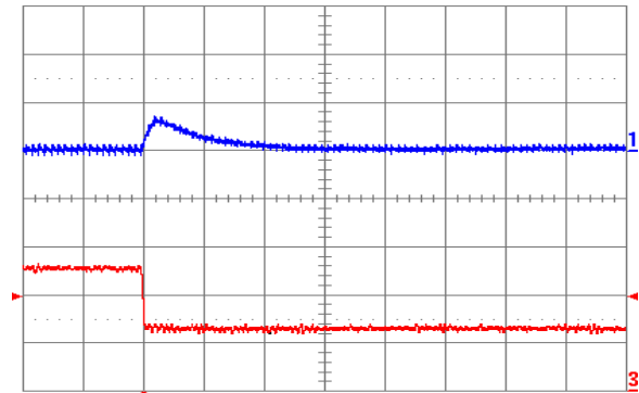
Fig. 1.5V.8: Output voltage response for V_{out} = 1.5\text{ V} to negative load current step change from 5 A to 2.5 A with slew rate of -5\text{ A}/\mu\text{s} at V_{in} = 12\text{ V} . Top trace: output voltage (100 mV/div.); Bottom trace: load current (2 A/div.). C_o = 47\text{ }\mu\text{F} ceramic. Time scale: 20\text{ }\mu\text{s}/\text{div} .
