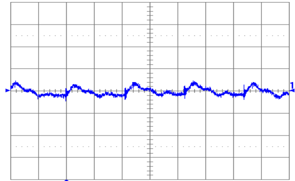
Fig. 1.5V.6: Output voltage ripple (20 mV/div.) at full rated load current into a resistive load with external capacitance 47\text{ }\mu\text{F} ceramic + 1\text{ }\mu\text{F} ceramic, and V_{in} = 12\text{ V} for V_{out} = 1.5\text{ V} . Time scale: 1\text{ }\mu\text{s}/\text{div} .
