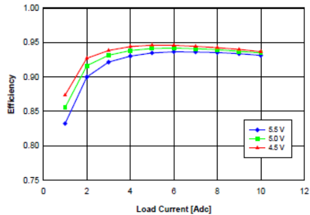
Fig. 2.5V.3: Efficiency vs. load current and input voltage for YNL05S10025 converter mounted vertically with air flowing at a rate of 200 LFM (1 m/s) and T_a = 25 ^{\circ} C.
