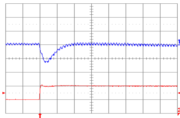
Fig. 1.2V.7: Output voltage response (YNL05S10012) to positive load current step change from 5 A to 10 A with slew rate of 5\ \text{A}/\mu\text{s} at V_{in} = 5\ \text{V} . Top trace: output voltage (100 mV/div.); Bottom trace: load current (5 A/div.). C_o = 47\ \mu\text{F} ceramic + 1\ \mu\text{F} ceramic. Time scale: 20 \mu\text{s} /div.
