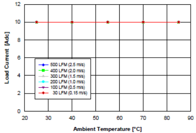
Fig. 2.5V.2: Available load current vs. ambient temperature and airflow rates for YNL05S10025 converter mounted horizontally with V_{in} = 5 V, and maximum MOSFET temperature \leq 110 ^{\circ} C.
