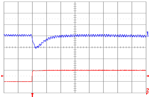
Fig. 2.5V.7: Output voltage response (YNL05S10025) to positive load current step change from 5 A to 10 A with slew rate of 5 A/ \mu\text{s} at V_{in} = 5\text{ V} . Top trace: output voltage 47 \mu\text{F} ceramic + 1 \mu\text{F} ceramic. Time scale: 20 \mu\text{s} /div.
