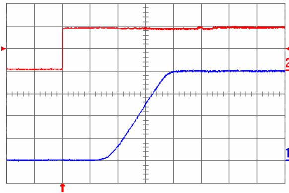
Fig. 2.0V.5: Turn-on transient (YNL05S10020) with the application of Enable signal at full rated load current (resistive) and 47 \mu\text{F} external capacitance at V_{in} = 5\text{ V} . Top (500 mV/div.); Time scale: 2 ms/div.
