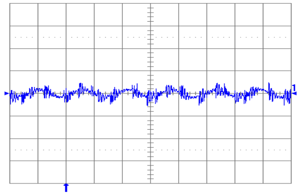
Fig. 2.0V.6: Output voltage ripple (20 mV/div.) at full rated load current into a resistive load with external capacitance 47 \mu\text{F} ceramic + 1 \mu\text{F} ceramic and V_{in} = 5\text{ V} (YNL05S10020). Time scale: 2 \mu\text{s} /div.
