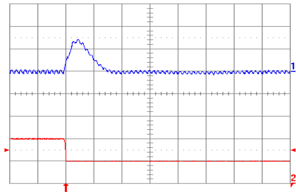
Fig. 2.0V.8: Output voltage response (YNL05S10020) to negative load current step change from 10 A to 5 A with slew rate of 5 A/ \mu\text{s} at V_{in} = 5\text{ V} . Top trace: output voltage (100 mV/div.); Bottom trace: load current (5 A/div.). C_o = 47\ \mu\text{F} ceramic + 1 \mu\text{F} ceramic. Time scale: 20 \mu\text{s} /div.
