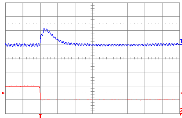
Fig. 2.5V.8: Output voltage response (YNL05S10025) to negative load current step change from 10 A to 5 A with slew rate of -5 A/ \mu\text{s} at V_{in} = 5\text{ V} . Top trace: output voltage 47 \mu\text{F} ceramic + 1 \mu\text{F} ceramic. Time scale: 20 \mu\text{s} /div.
