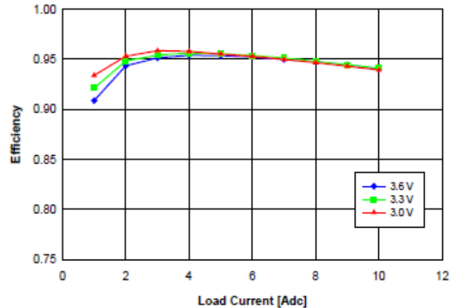
Fig. 2.5V.4: Efficiency vs. load current and input voltage for YNL05S10025 converter mounted vertically with air flowing at a rate of 200 LFM (1 m/s) and T_a = 25 ^{\circ} C.
