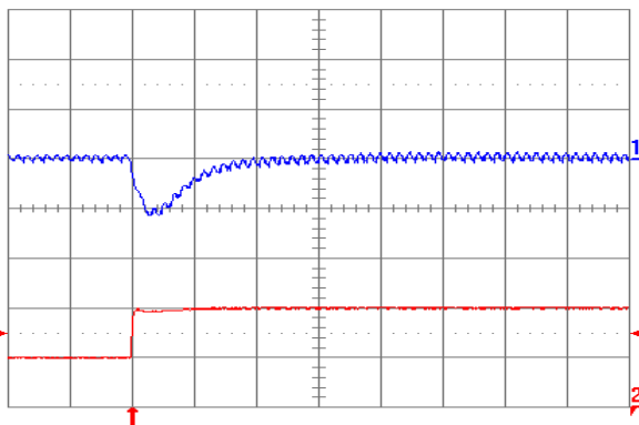
Fig. 2.0V.7: Output voltage response (YNL05S10020) to positive load current step change from 5 A to 10 A with slew rate of 5 A/ \mu\text{s} at V_{in} = 5\text{ V} . Top trace: output voltage (100 mV/div.); Bottom trace: load current (5 A/div.). C_o = 47\ \mu\text{F} ceramic + 1 \mu\text{F} ceramic. Time scale: 20 \mu\text{s} /div.
