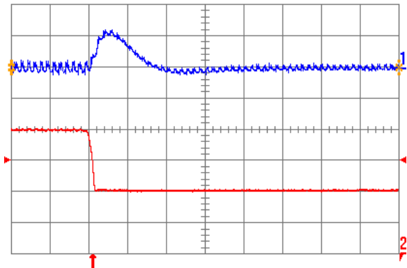
Fig. 3.3V.7: Output voltage response for V_{out} = 3.3\text{ V} to negative load current step change from 20 A to 10 A with slew rate of -5\text{ A}/\mu\text{s} at V_{in} = 12\text{ V} . Top trace: output voltage (200 mV/div.); Bottom trace: load current (5 A/div.). C_o = 100\ \mu\text{F} ceramic. Time scale: 20 \mu\text{s} /div.
