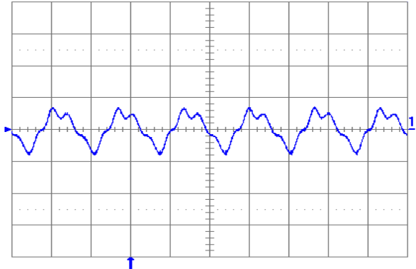
Fig. 3.3V.5: Output voltage ripple (20 mV/div.) at full rated load current into a resistive load with external capacitance 100\ \mu\text{F} ceramic + 1\ \mu\text{F} ceramic and V_{in} = 12\text{ V} for V_{out} = 3.3\text{ V} . Time scale: 2 \mu\text{s} /div.
