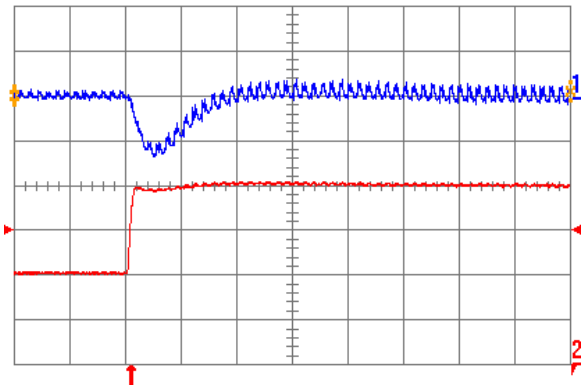
Fig. 3.3V.6: Output voltage response for V_{out} = 3.3\text{ V} to positive load current step change from 10 A to 20 A with slew rate of 5\text{ A}/\mu\text{s} at V_{in} = 12\text{ V} . Top trace: output voltage (200 mV/div.); Bottom trace: load current (5 A/div.). C_o = 100\ \mu\text{F} ceramic. Time scale: 20 \mu\text{s} /div.
