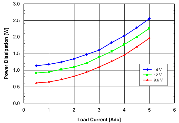
Fig. 5.0V.4: Power Loss vs. load current and input voltage for V_{out} = 5.0V converter mounted vertically with air flowing from pin 5 to pin 1 at a rate of 200 LFM (1 m/s) and T_a = 25^\circ C .
