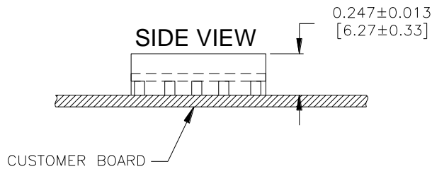
YM12S Pinout (Surface Mount)
