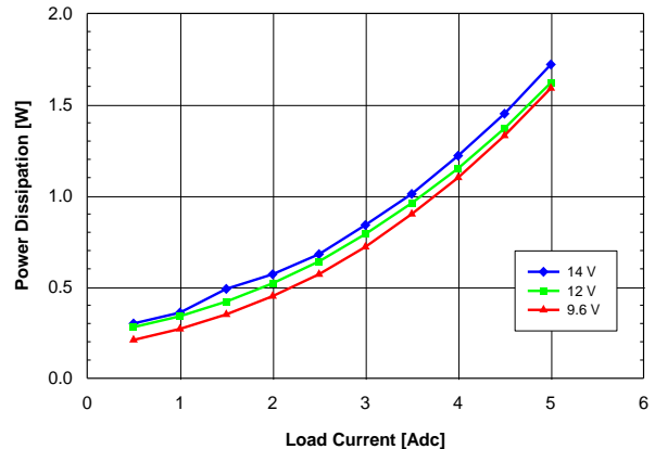
Fig. 1.2V.4: Power Loss vs. load current and input voltage for V_{out} = 1.2V converter mounted vertically with air flowing from pin 5 to pin 1 at a rate of 200 LFM (1 m/s) and T_a = 25\text{ }^{\circ}C .
