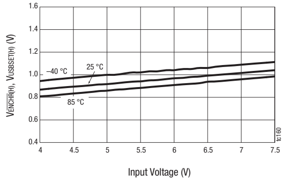
Figure 20. Input High Threshold vs Input Voltage
