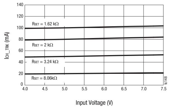
Figure 8. Preconditioning Charge Current vs Input Voltage
