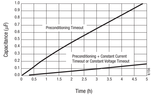
Figure 16. CT Pin Capacitance vs Counter Timeout
