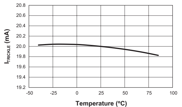
Preconditioning Charge Current vs. Temperature ( R_{SET} = 8.06k\Omega ; AAT3681A, AAT3681A-2, and AAT3681A-5 Only)
