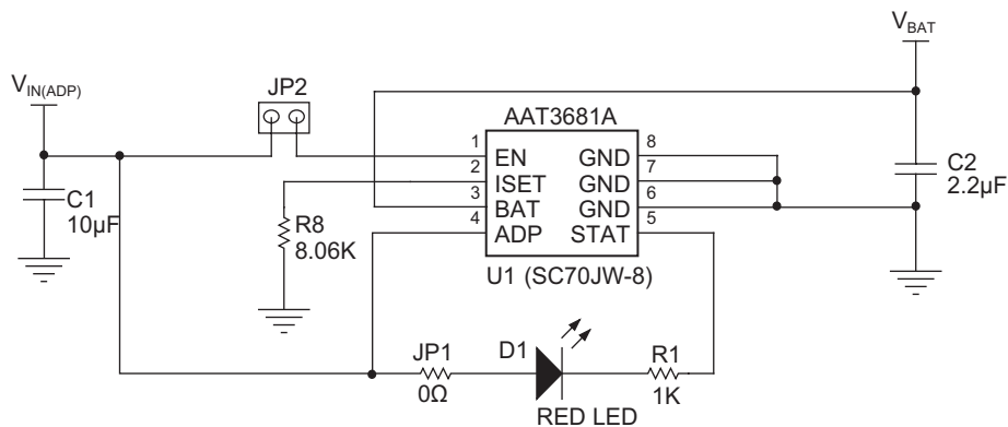
Figure 7: AAT3681A Evaluation Board Schematic Diagram.
