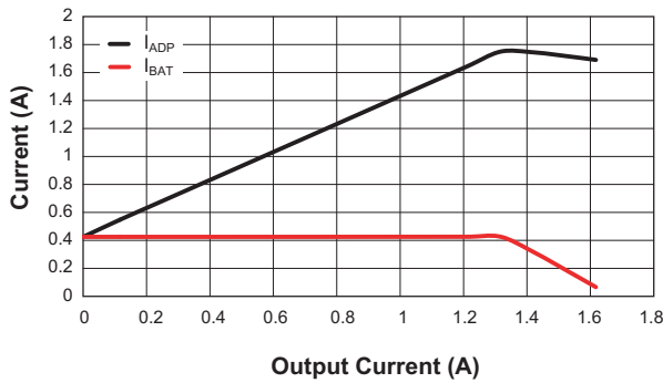
Adapter and Charging Current vs. Output Current
