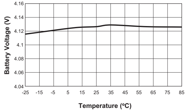
Recharge Voltage Threshold vs. Temperature (V ADP = 5V; R SET = 56.7kΩ)
