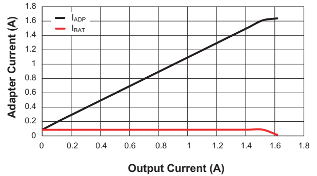
Adapter and Charging Current vs. Output Current
