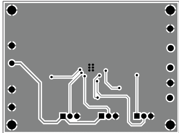
Figure 7: AAT3672-1/-2 Evaluation Board Bottom Layer.
