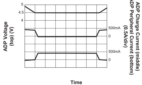
ADP Charge Current (500mA Charging Setting)
