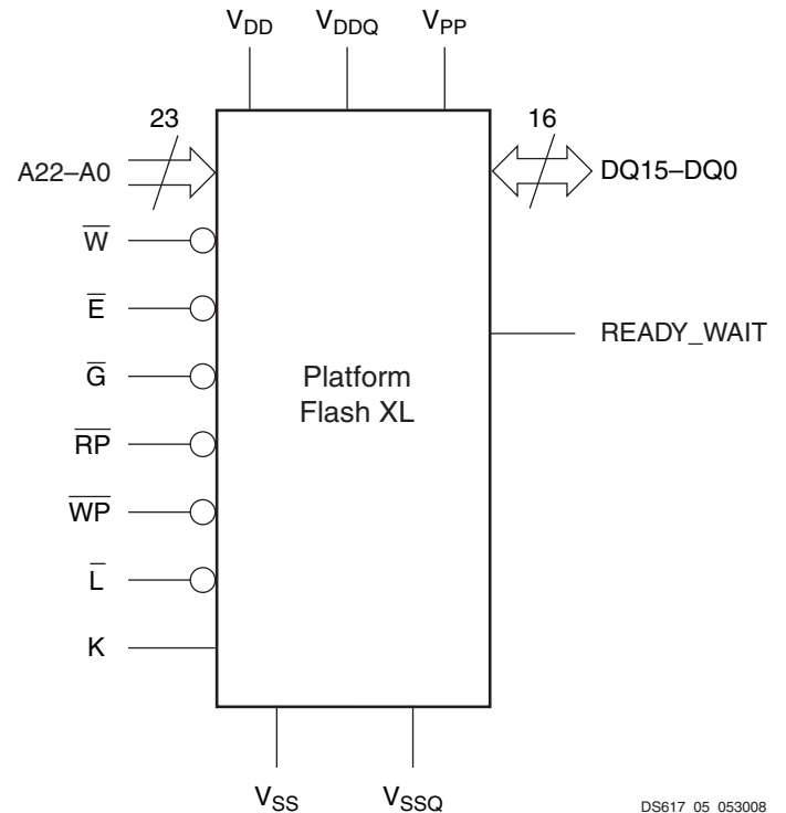
Figure 5: Logic Diagram
