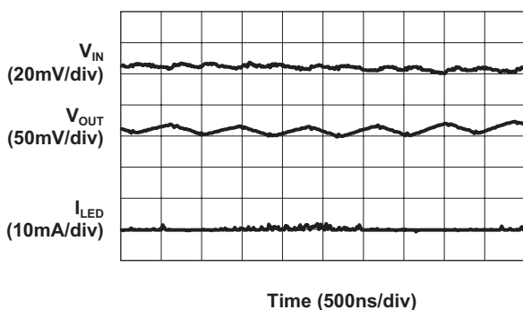
Load Characteristics ( V_{IN} = 3.3V ; 1.5X Mode; 10mA/ch Load)
