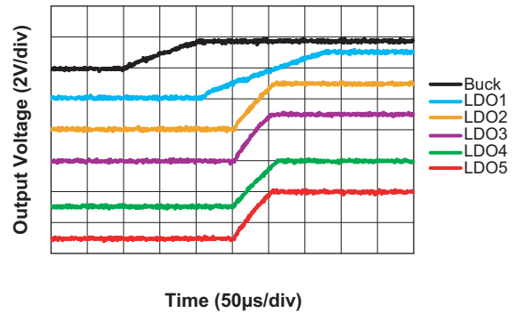
Start-up Sequence ( V_{CHGIN} = 5.0V )
