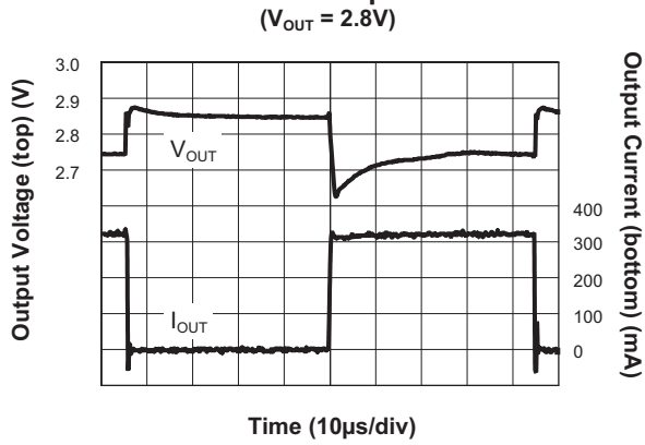
Load Transient Response 300mA
