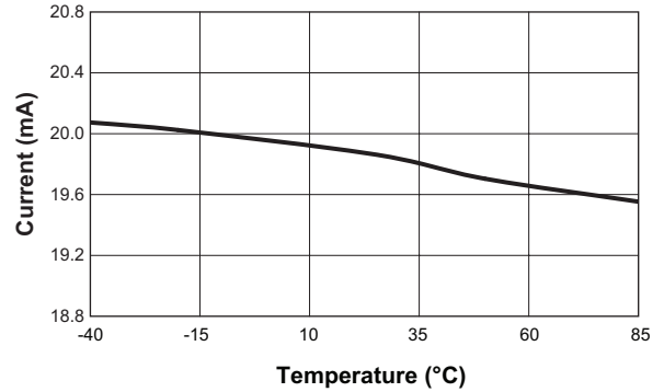
LED Current Accuracy vs. Temperature ( V_{IN} = 3.6V , R_{SET} = 15k\Omega )
