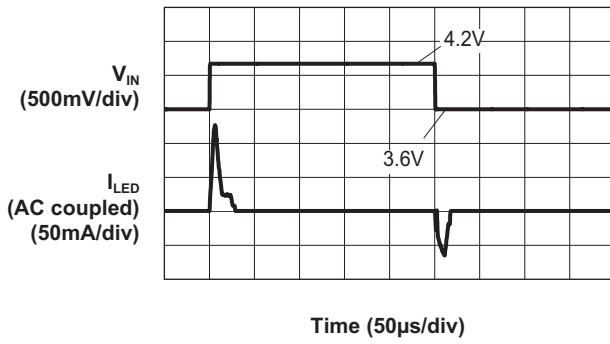
Movie Mode Line Transient (68.5mA/ch; V_{IN} = 4.2V to 3.6V )
