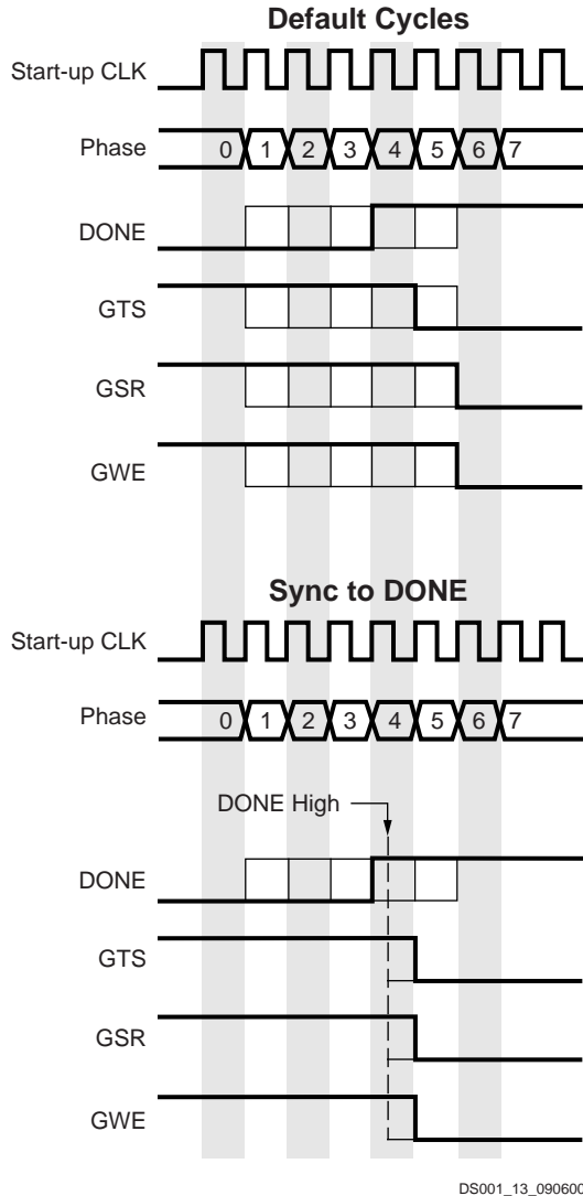
Figure 13: Start-Up Waveforms
