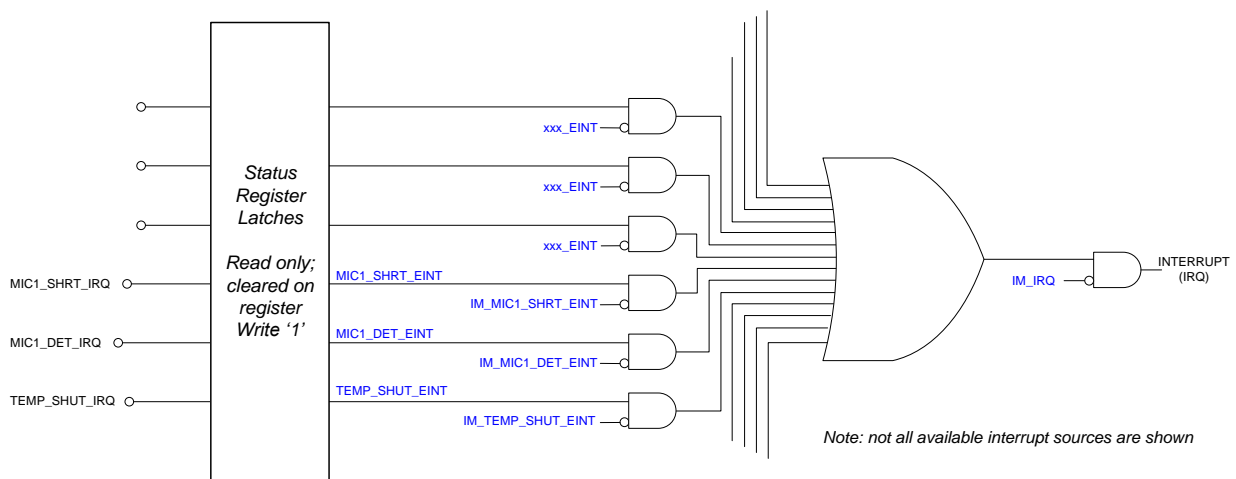
Figure 43 Interrupt Controller
