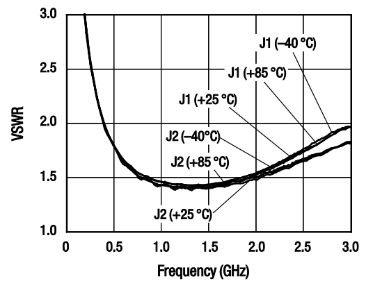
Figure 6. VSWR vs Frequency (32 dB State)
