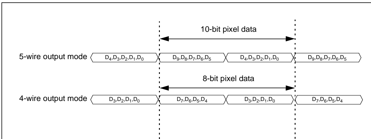
Figure 6: Digital data output modes
