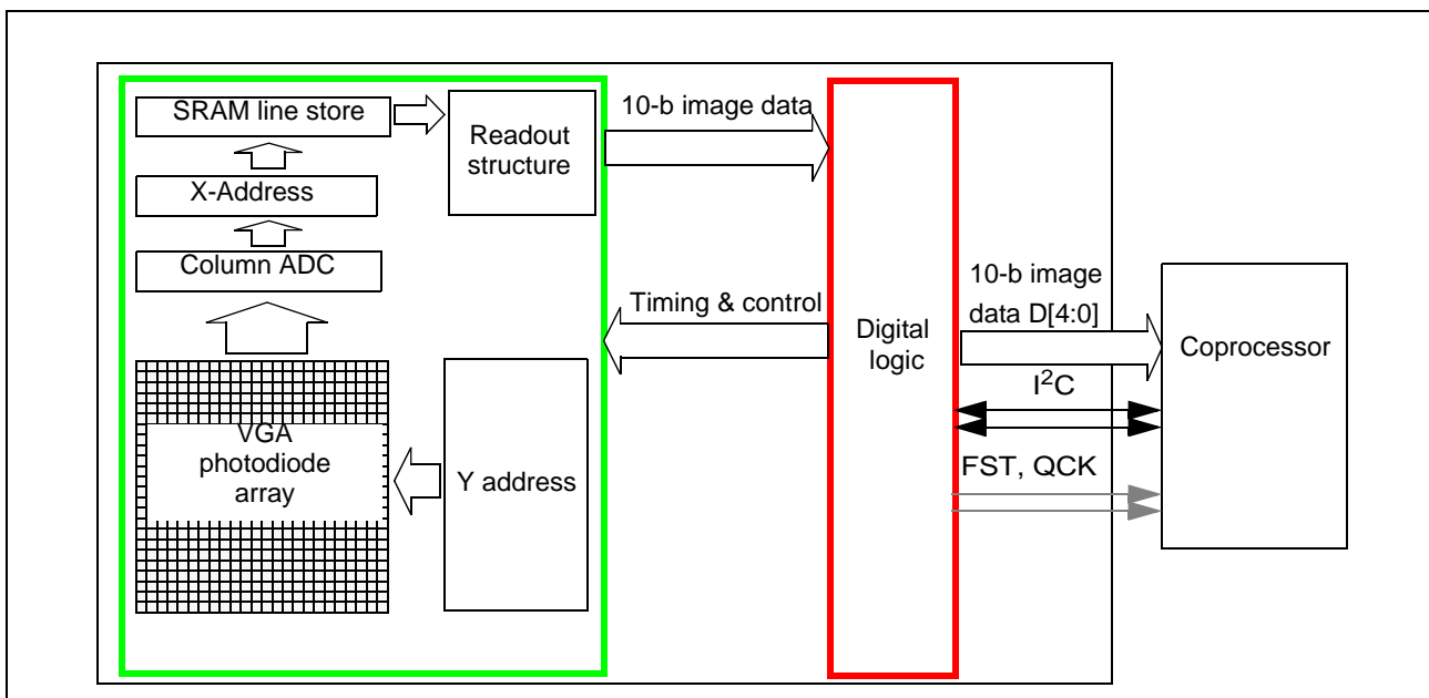
Figure 4: Overview of video block
