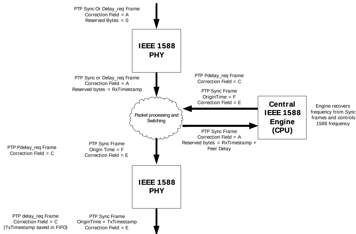
Figure 33 • One-Step E2E BC
