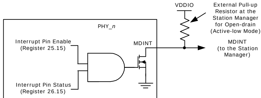
Figure 68 • MDINT Configured as an Open-Drain (Active-Low) Pin
